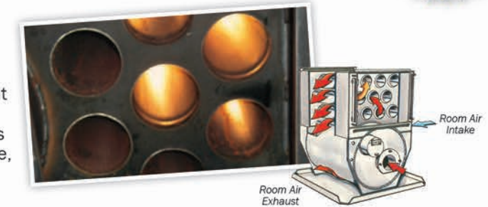
Our unique design causes a triple pass of heated exhaust air through heat exchanger tubes before exiting up the chimney. Maximum BTU transfer occurs as air passes over heat exchanger tubes and the firebox, providing high heat efficiency.
